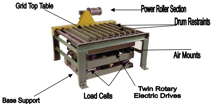
Model GWT Grid Deck Vibratory Weigh Scale Packer
