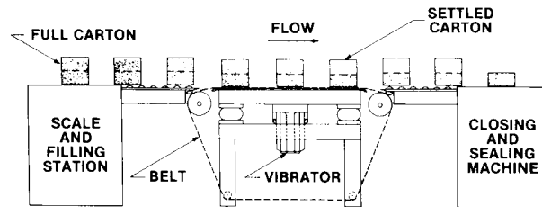
Typical Vibratory Belt Table Conveyor Installation
